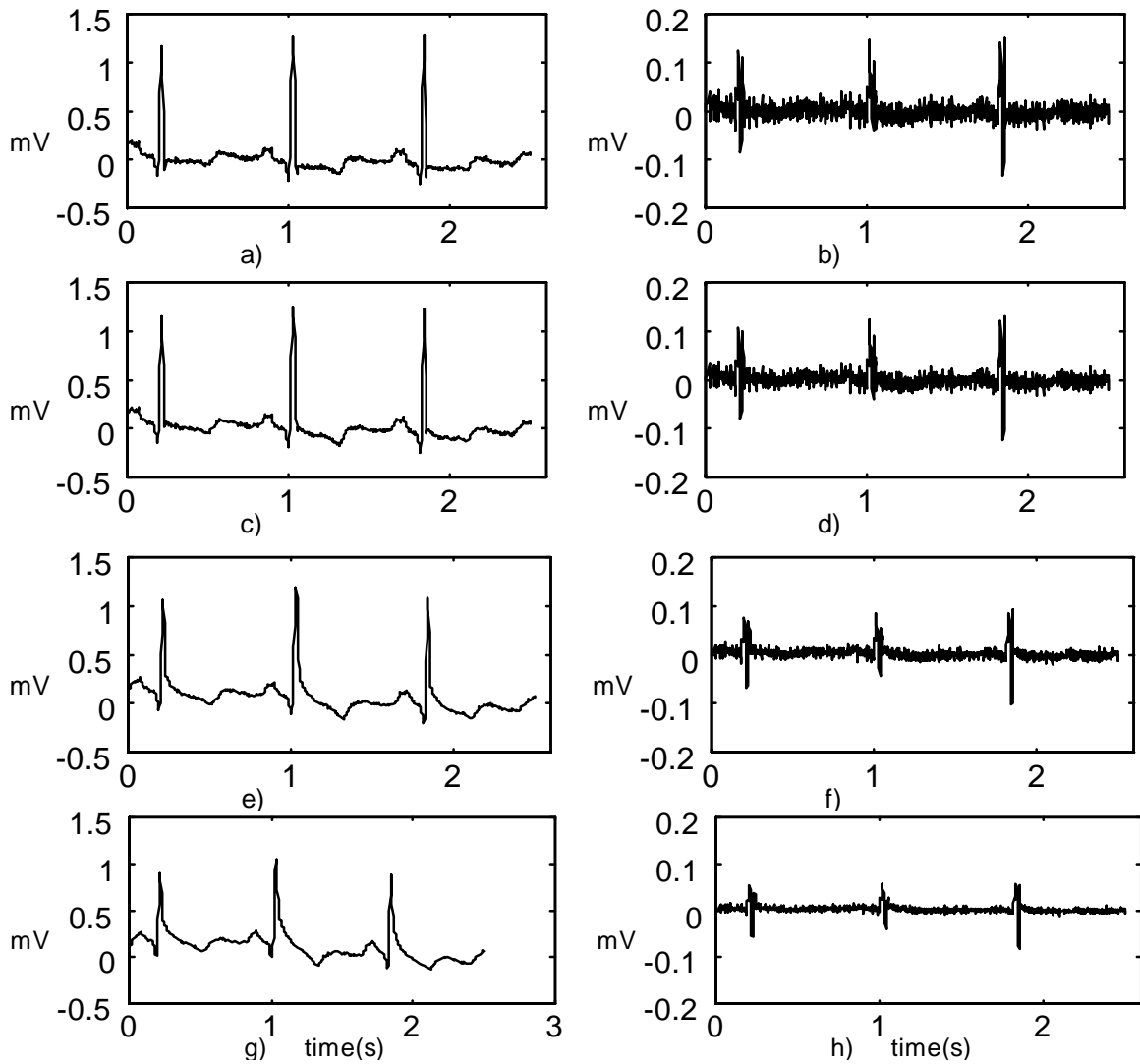
Fig. 2. a) original ECG and b) corresponding residual signal. c),e) and g) differentiated signals with n = -0.1, -0.3 and -0.45 , d),f),h) corresponding residual signals.
