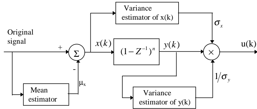
Fig. 1. Block diagram of the system used to reduce the variance of prediction error using fractional digital differentiation.
