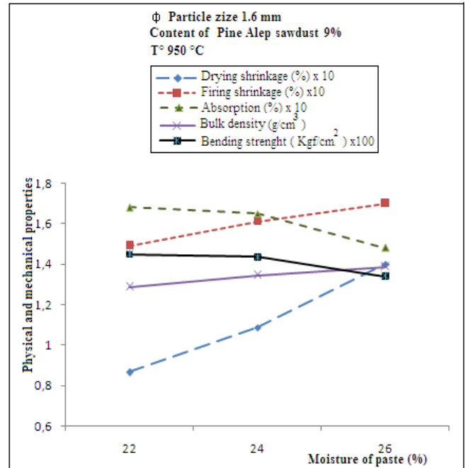
Fig. 3 Physical-mechanical properties in relation with moisture of mixtures according the particle size and Pine Alep content
