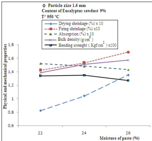
Fig. 2 Physical-mechanical properties in relation with moisture of mixtures according the particle size and Eucalyptus content
