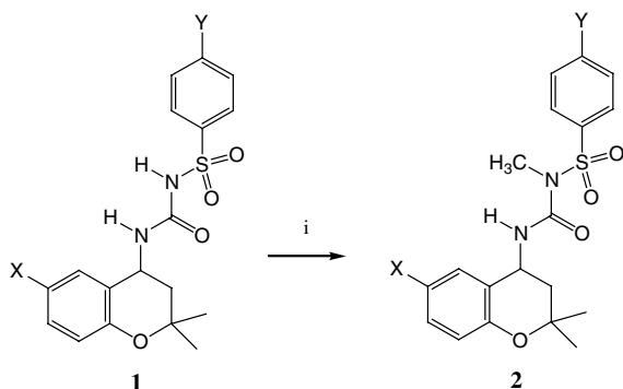
Scheme 1. Reagents: (i) CH 3 I or (CH 3 O) 2 SO 2 , Na 2 CO 3 , CH 3 CN.
